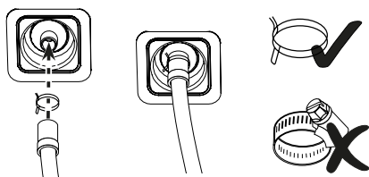
Fig. 47: Connecting the condensate drain hose
