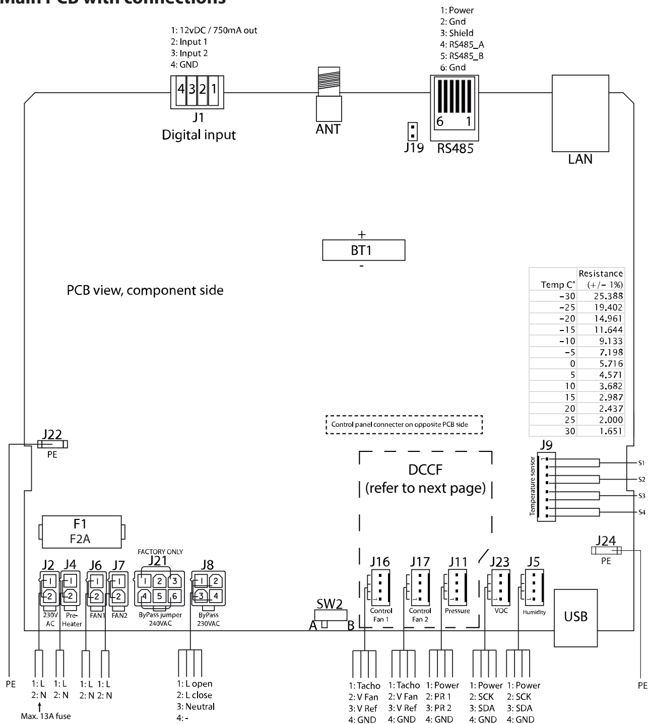
Fig. 62: Main PCB with connections
