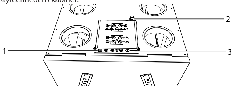
Fig. 20: Betjeningspanel
