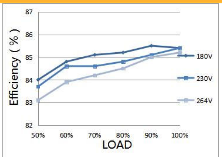
Fig.6 Efficiency-Load curve
