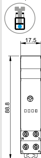
Type 14.81 Box clamp
