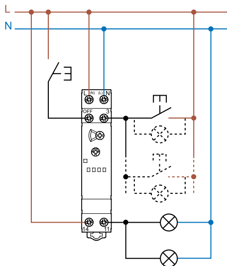
Type 14.11
