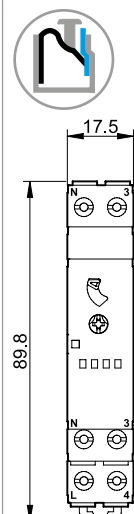
Type 14.61 Push-in terminal
