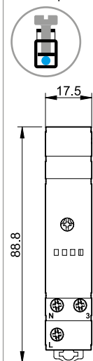
Type 14.91 Box clamp
