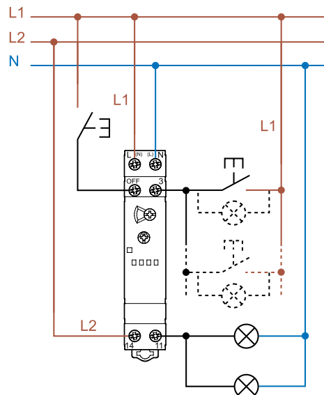
Type 14.11
