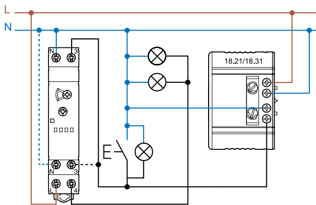
Type 14.01, 14.61 or 14.71
