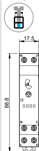
Type 14.71 Box clamp
