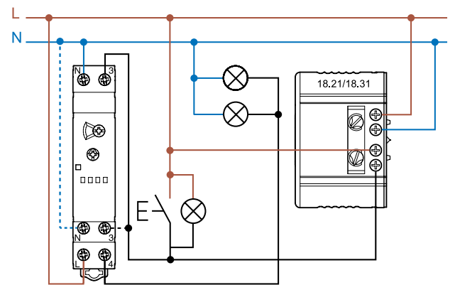
Type 14.01, 14.61 or 14.71
