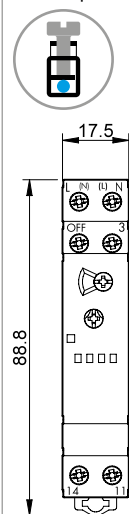
Type 14.11 Box clamp
