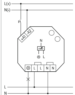
Universal control voltage 8..230V UC, supply voltage and switching voltage 230V
