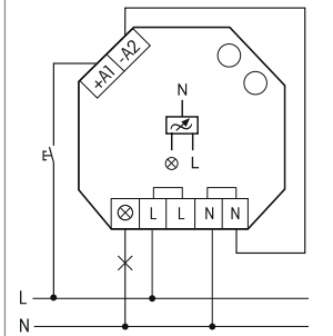
Control voltage, supply voltage and switching voltage 230V
