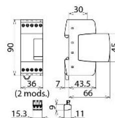
Dimension drawing DR M 4P 255 FM
