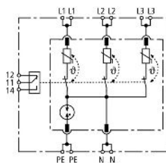
Basic circuit diagram DR M 4P 255 FM
