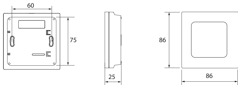
Rumtermostat Danfoss Icon2™ / 24V RT 088U2128
