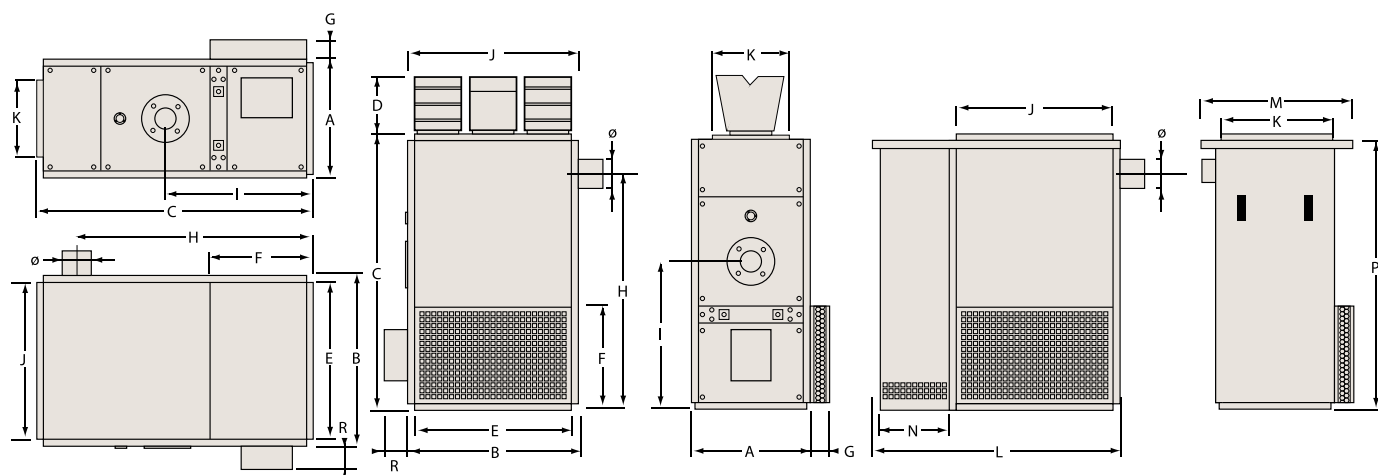
Vandret version
