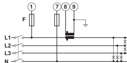
Fig. 6 AV5 balanced load
