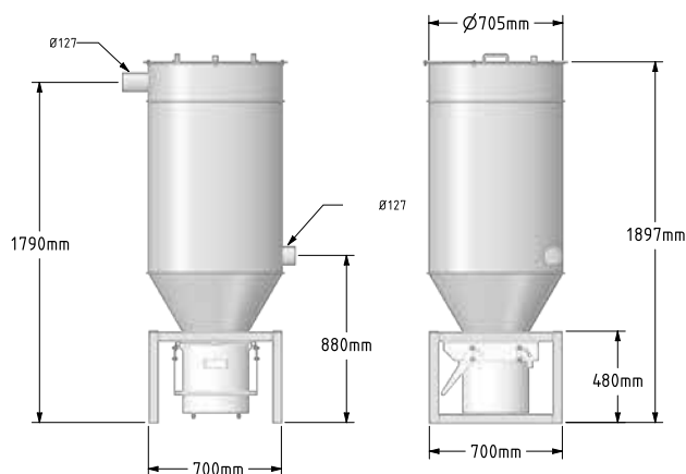
03-956A HVU FilterCyclon
