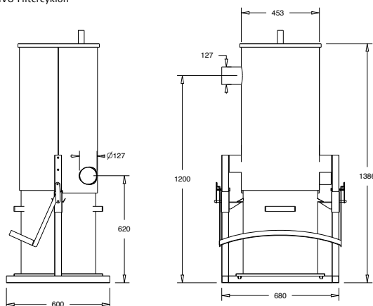
03-956 HVU Filtercyclon
