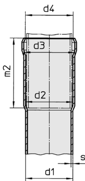
Lang muffe 2A Lang muffe 2A
