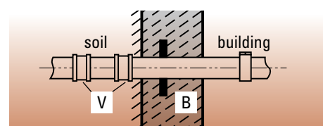
SML pipe with wall flange
