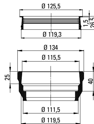
WC-socket for plastic pipe connection DN 100 item no. rubber joints separately: 100000
