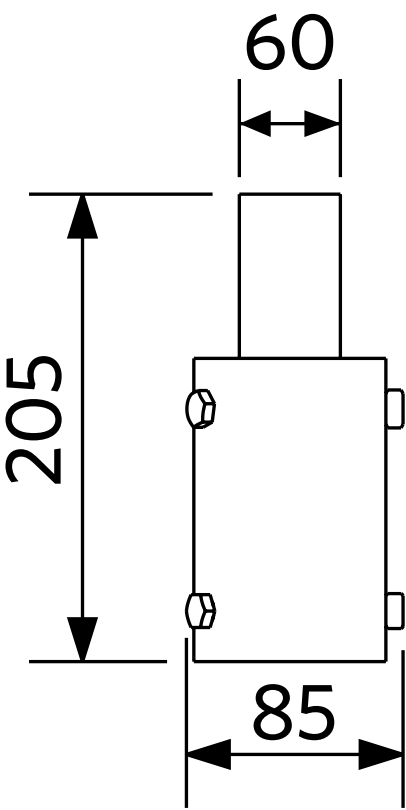
LEDStreetlight 76-Adapter-60
