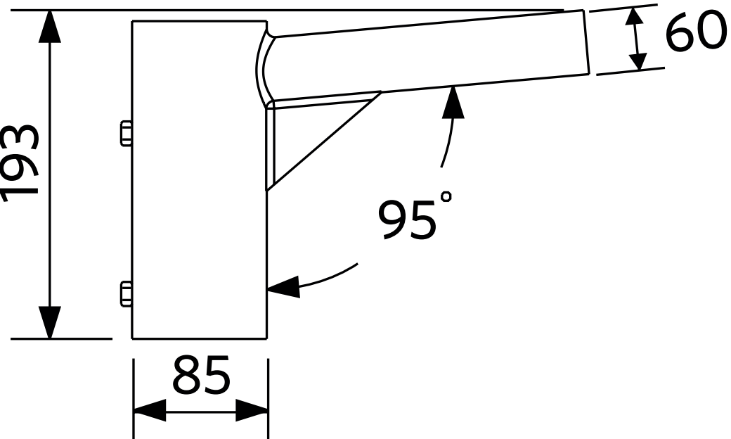
LEDStreetlight Pole-Top-76-Adapter-60
