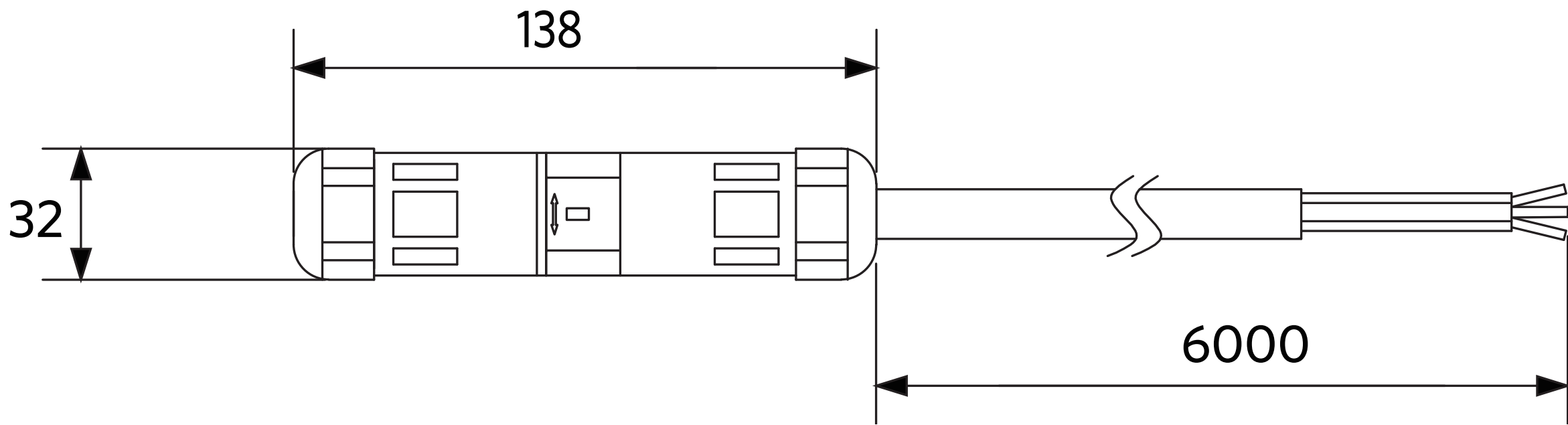
LEDStreet-SE-ExtensionCable
