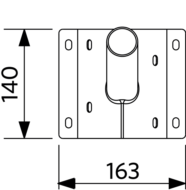
LEDStreetlight Wall-Bracket-60
