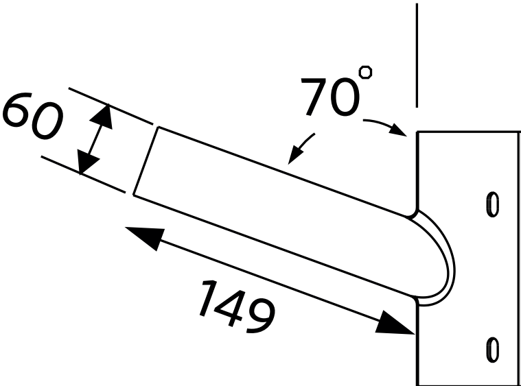
LEDStreetlight Wall-Bracket-60
