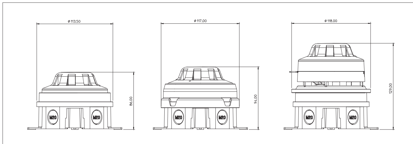
Figure 2: Dimensions
