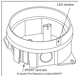
Fig 1 Mounting Box
