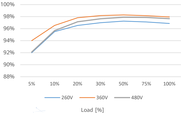
Efficiency Curve
