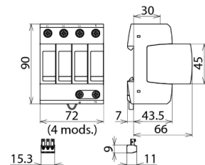
Dimension drawing DG M TNS 275 FM
