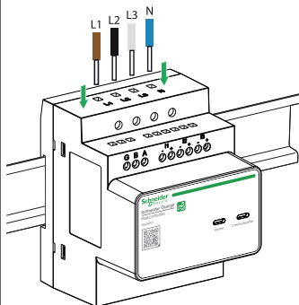
230V AC 3-Phasen
