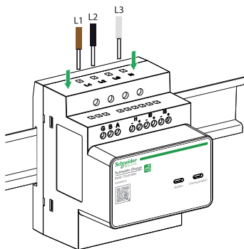
230V AC 3-Phase No Neutral
