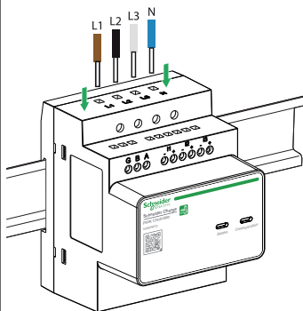
230V AC 3-Phase
