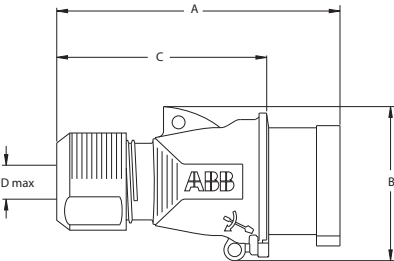
Dimensions (mm)
