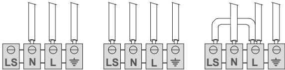
Connection diagram
