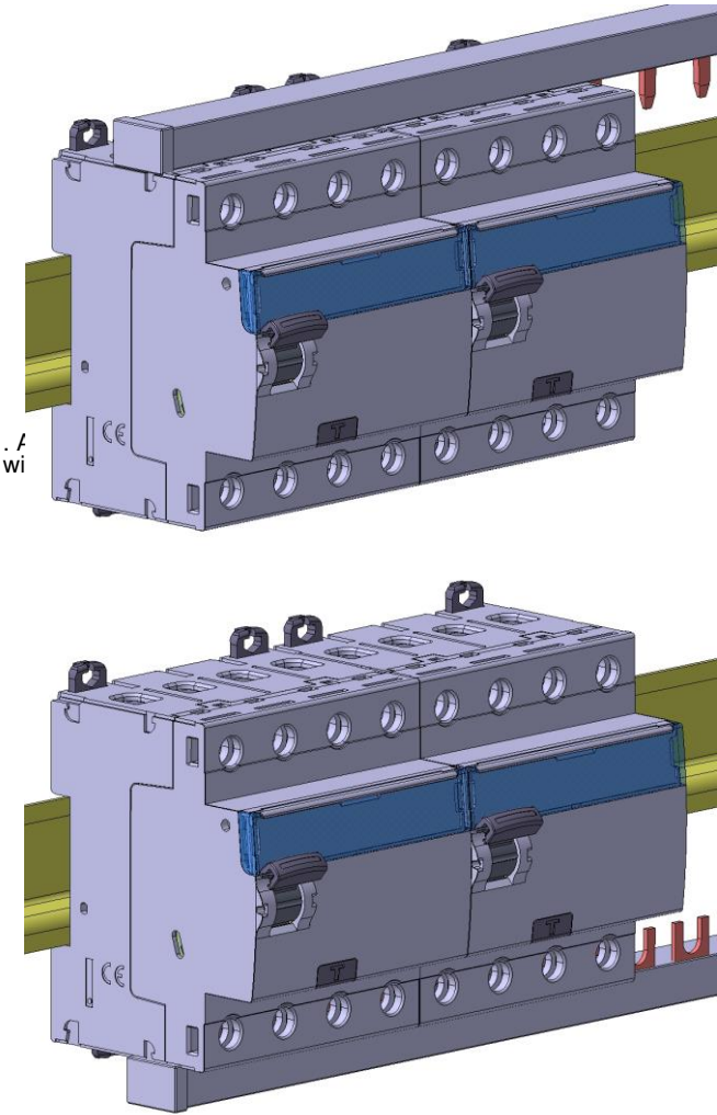
Prong busbar
