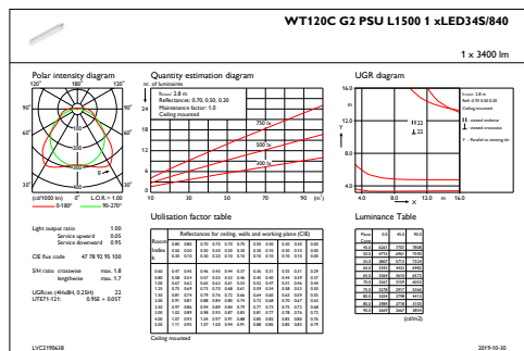
IFGU1_WT120CG2PSUL15001xLED34S840
