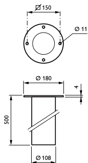
Smart LED bollard II acc. ZCP150
