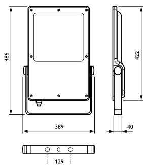
CoreLine Tempo BVP110/120/125/130
