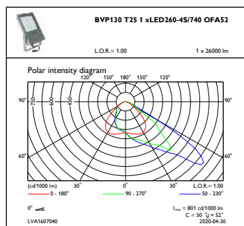
OFPC1_BVP130T251xLED260-4S740OFA52
