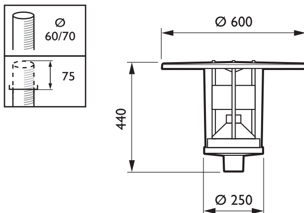
BPS962 GRN29/830 DF CLO-DDF6 C4K
