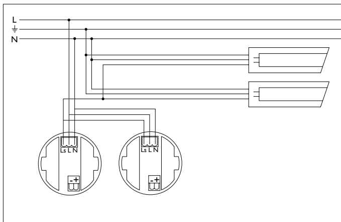
Parallelinstallation
