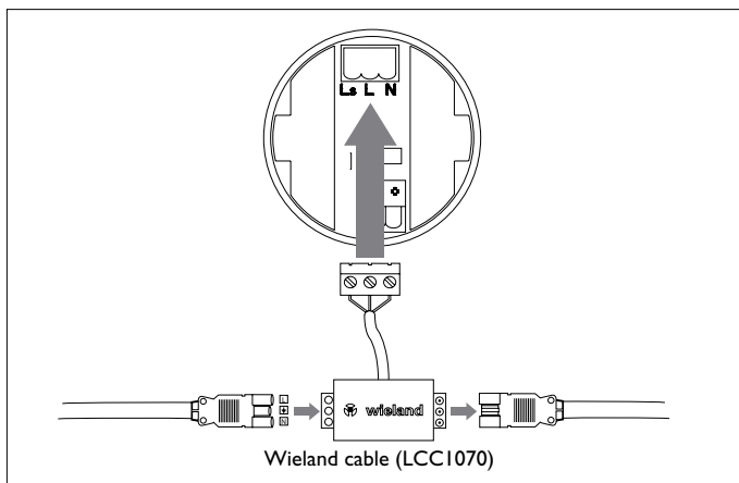
Installation (Wieland)
