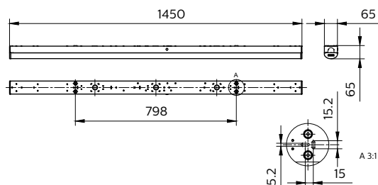
BN126C LED52S/840 PSU L1500
