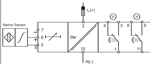
PMC01D - Namur sensor input
