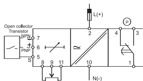
PMC01C - Open collector input
