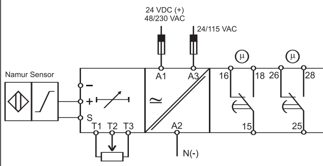
DMC01D - Namur sensor input
