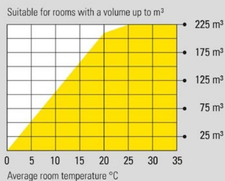
Room size suitability of the DH 15 for keeping dry
