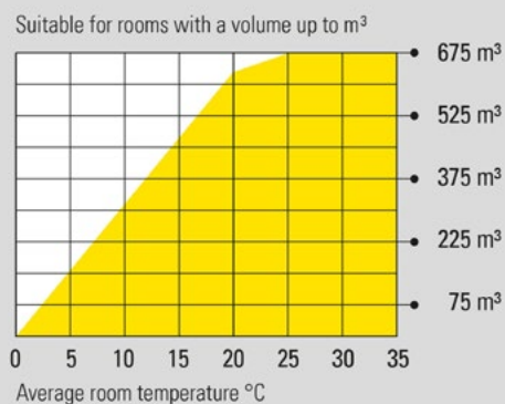
Room size suitability of the DH 60 for keeping dry
