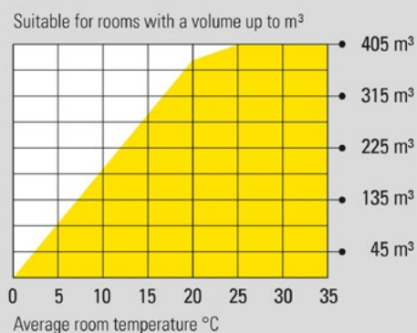
Room size suitability of the DH 30 for keeping dry
