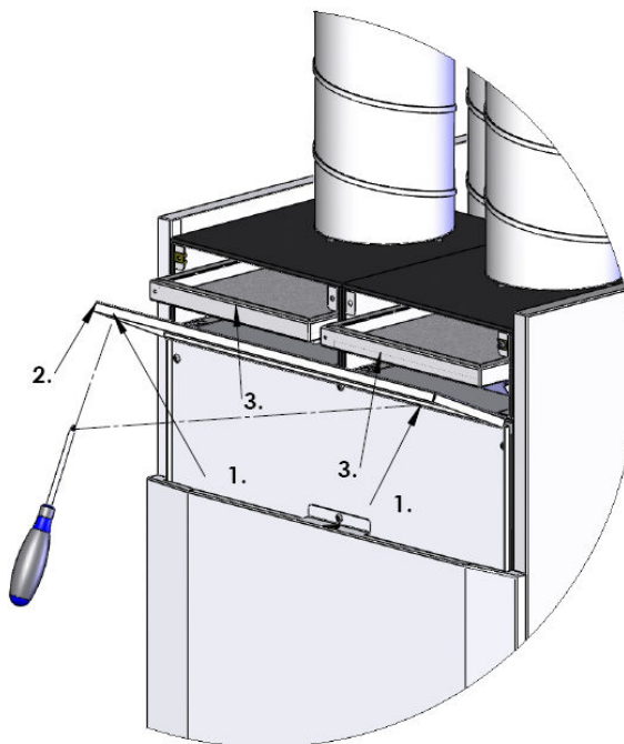
Figur 20: Filterskift
